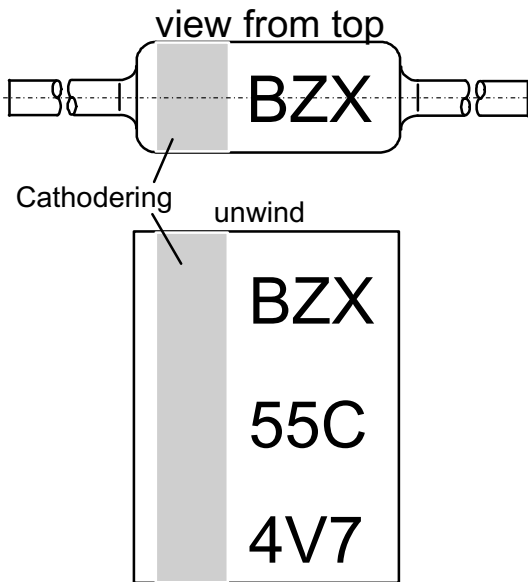
Figure 12. SOD-64
