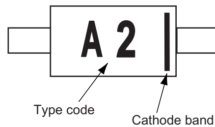
Figure 6. SOD-323
