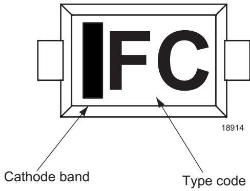
Figure 7. SOD-523
