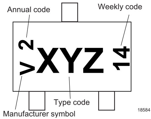
Figure 9. SOT-23
