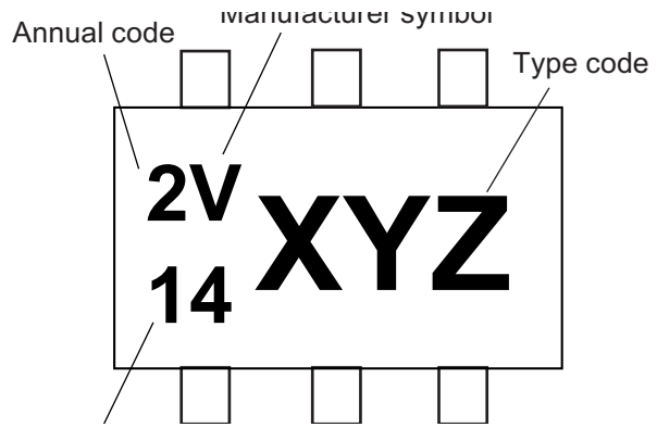
Figure 10. SOT-363
