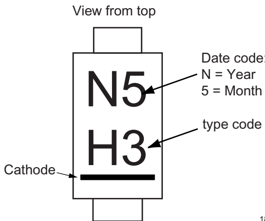
Figure 3. SMF (DO-219AB)
