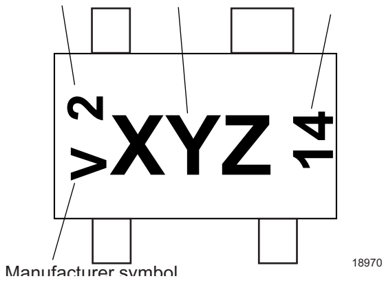
Figure 8. SOT-143
