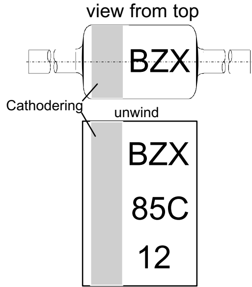
Figure 14. DO-41
