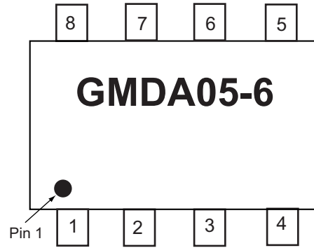
Figure 4. SO-8
